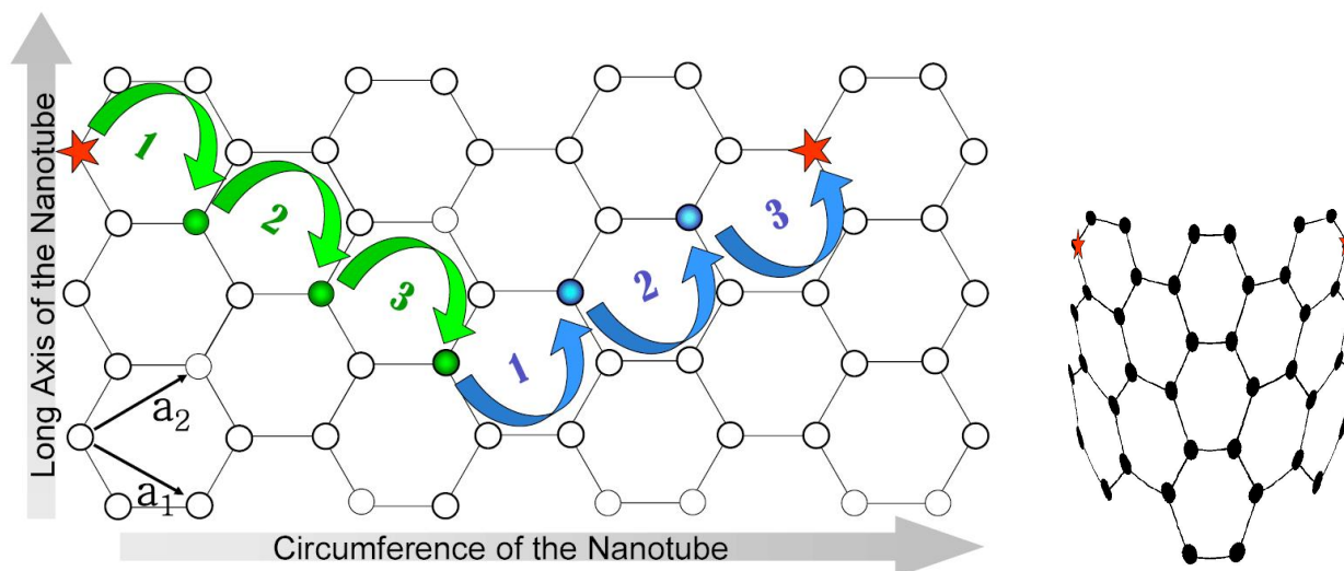
Figure 3. Counting a (3,3) armchair nanotube. The red stars represent the same carbon atom; the stars would overlap if you were to “roll” the graphene sheet into a tube.
