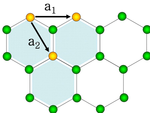
Figure 1. The counting directions ( \mathbf{a}_1 and \mathbf{a}_2 ) point from an arbitrary “origin” atom towards the closest equivalent carbon atoms in the graphene lattice.
