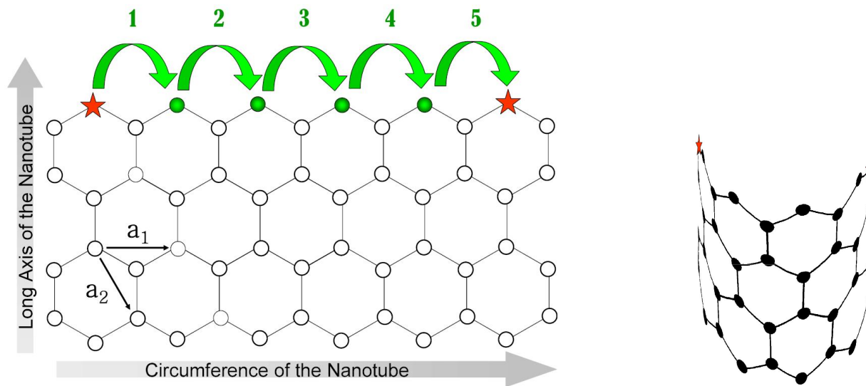
Figure 2. Counting a (5,0) zig-zag nanotube. The red stars represent the same carbon atom; the stars would overlap if you were to “roll” the graphene sheet into a tube.
