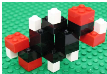
terephthalic acid
