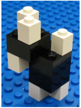
propylene (propene)
