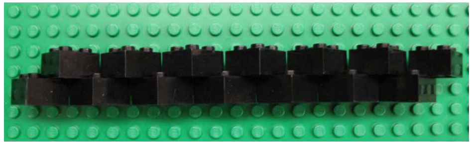
propylene (propene)
